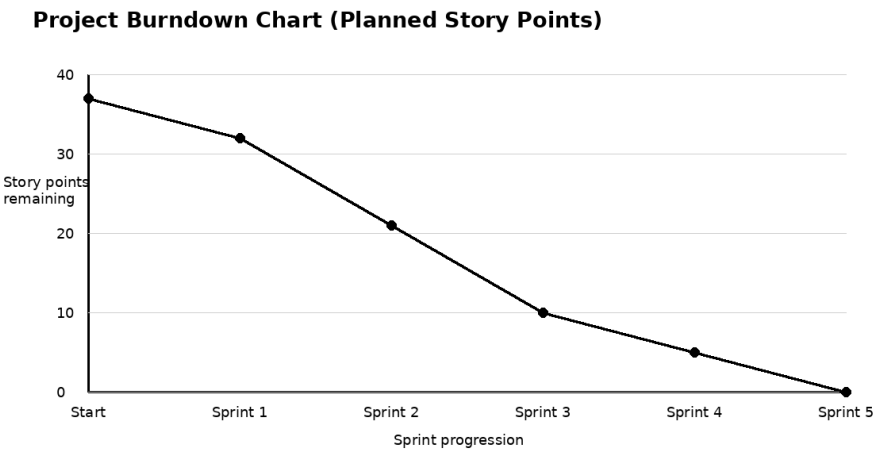
Figure 1: Planned project burndown based on the estimated 37 story points.
